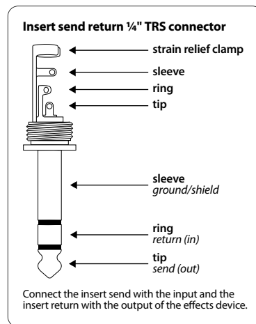
Fig. 5.7: Insert send and return ¼" TRS connector
