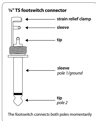
Fig. 5.5: ¼" TRS footswitch connector
