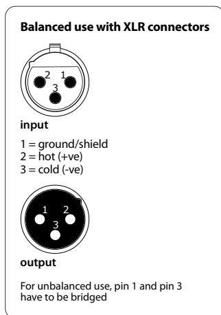
Fig. 5.4: XLR connectors
