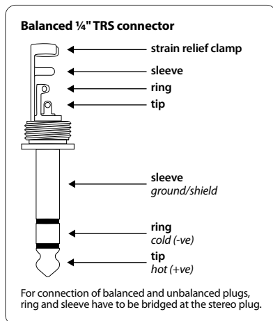
Fig. 5.2: ¼" TRS connector
