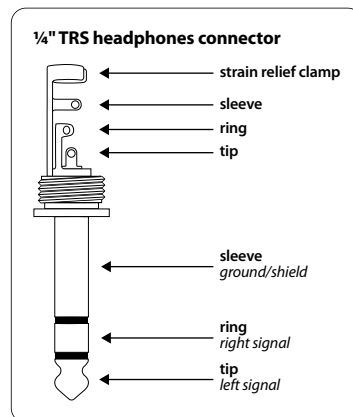
Fig. 5.6: ¼" TRS connector for headphones
